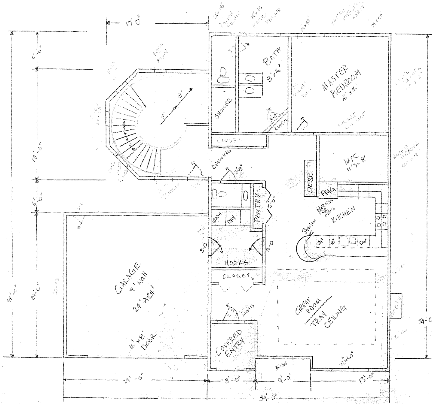
SPHS 16-17 FLOOR PLAN 1/4" = 1'
